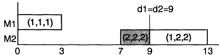
Figure 21. Resulting schedule after Earliness Reduction Procedure for figures 15's schedule
